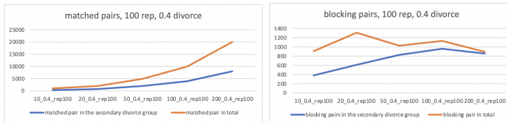
Figure 2: blocking pairs and matched pairs
