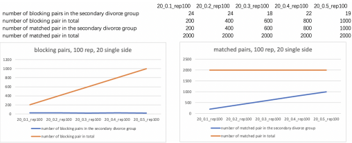
Figure 4: matching pairs and blocking pairs
