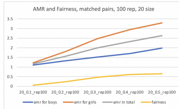
Figure 3: AMR and fairness
