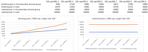
Figure 6: AMR and fairness
