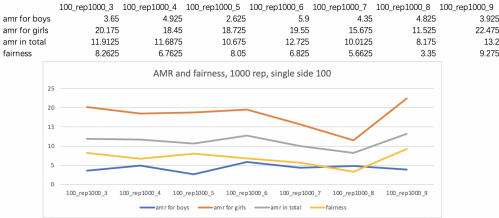
Figure 5: AMR and fairness
